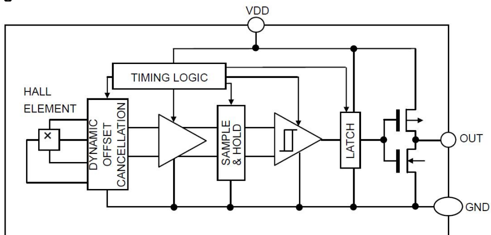
Figure 3, Block Diagram of AS1919
