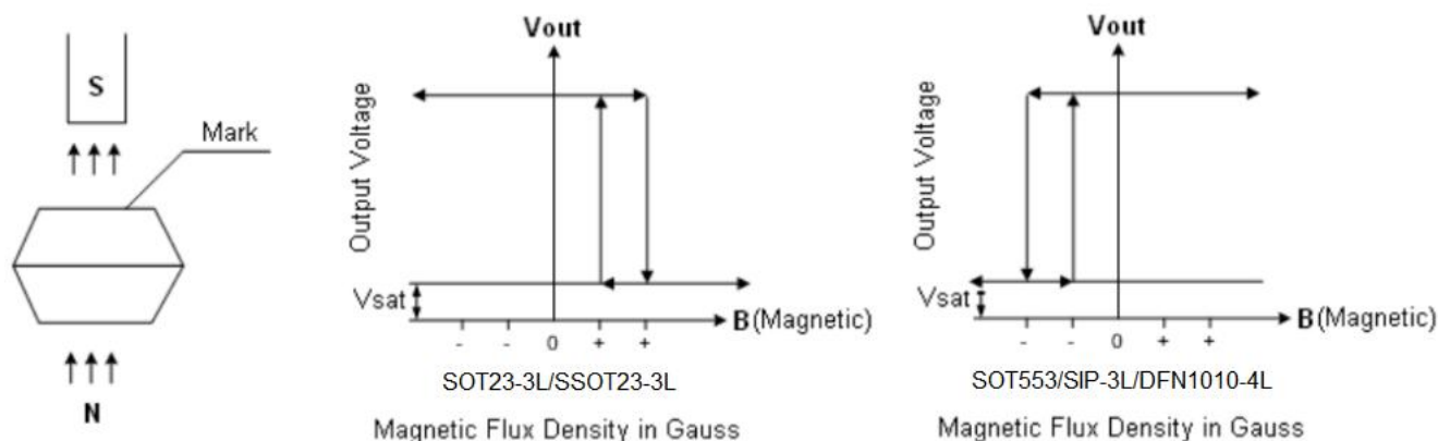
Fig 4, Magnetic Operation Characteristic of AS1919
