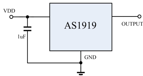
Figure 1, Typical Application Circuit of AS1919
